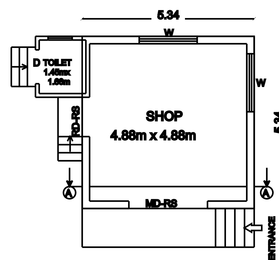
FLOOR PLAN
