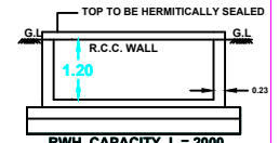
RW SECTION
