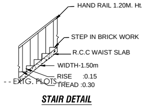
STAIR DETAIL
