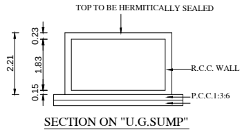
SECTION ON "U.G.SUMP"
