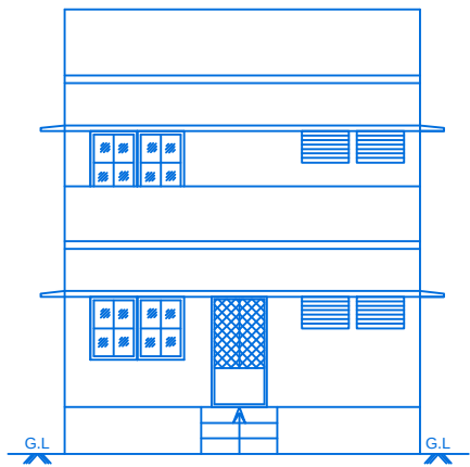
FRONT ELEVATION
