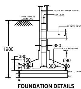
FOUNDATION DETAILS
