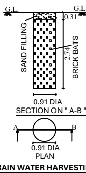
RAIN WATER HARVESTING
