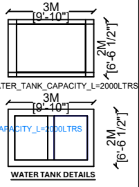
WATER TANK DETAILS
