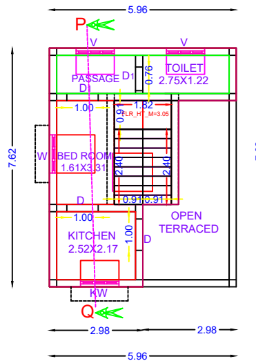
FIRST FLOORPLAN
