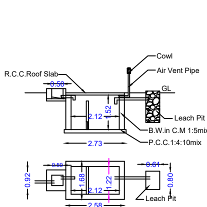
DETAILS OF SEPTIC TANK
