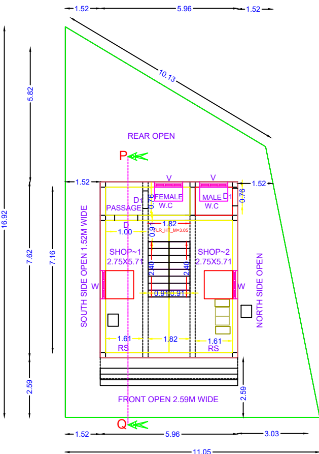
GROUND FLOORPLAN
