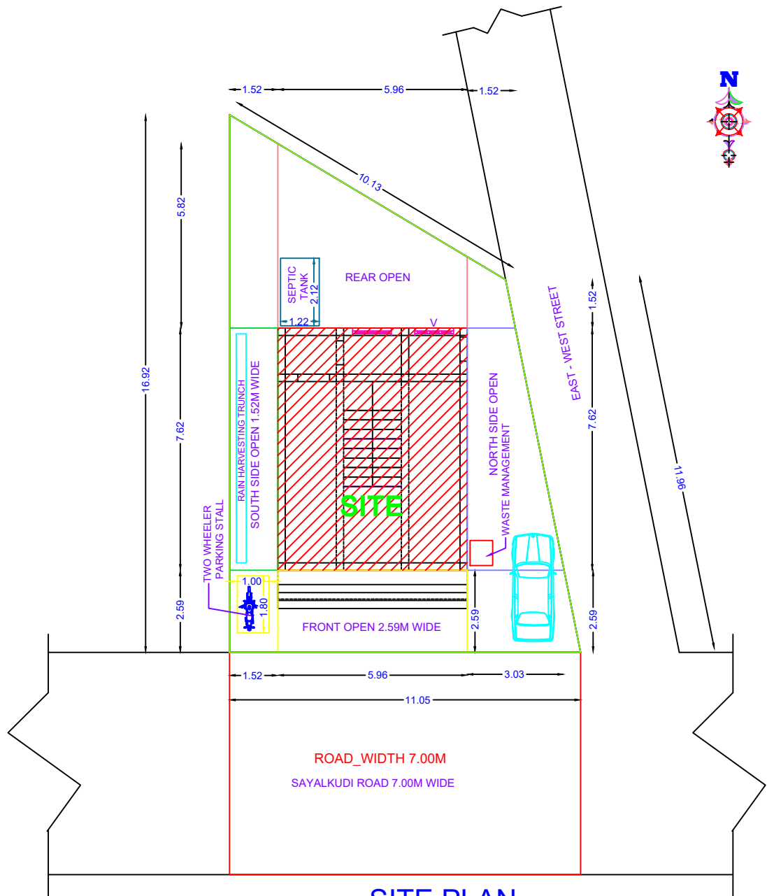
SITE PLAN
