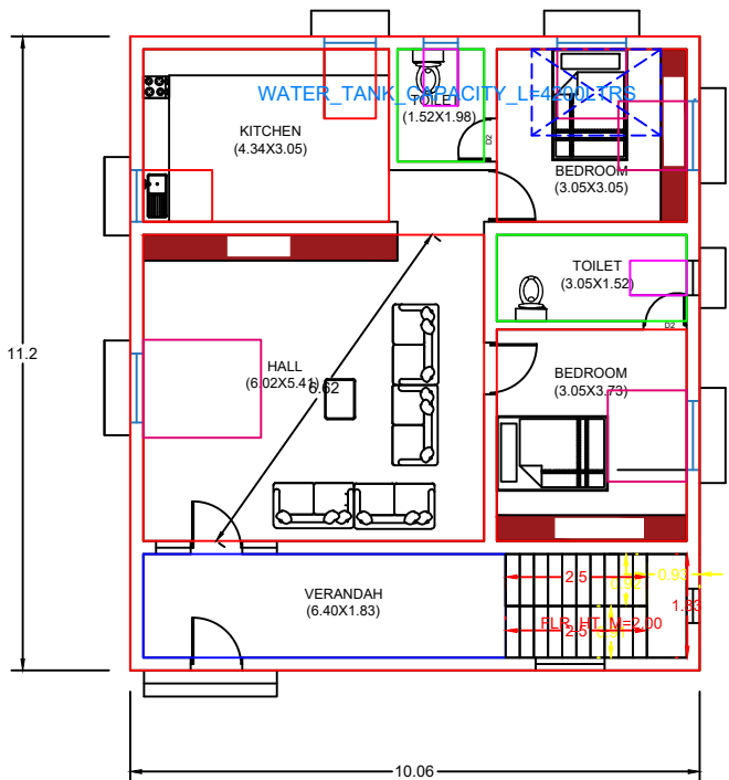
RAIN WATER HARVESTING SYSTEM RWHT CAPACITY=1000LTRS
