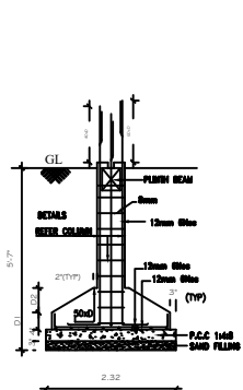
SCALE : 1:50 FOUNDATION DETAILS
