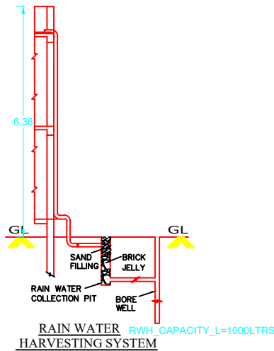
RAIN WATER HARVESTING SYSTEM RWHT CAPACITY=1000LTRS
