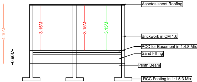
SECTION
