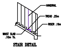
STAIR DETAIL
