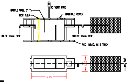
SEPTIC TANK AND TRENCH & U TRAP
