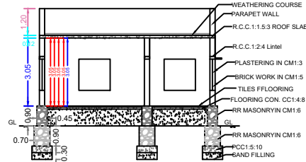
SECTION ON 'XY'
