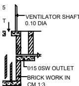
SEPTIC TANK
