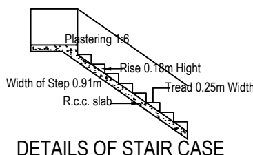
DETAILS OF STAIR CASE
