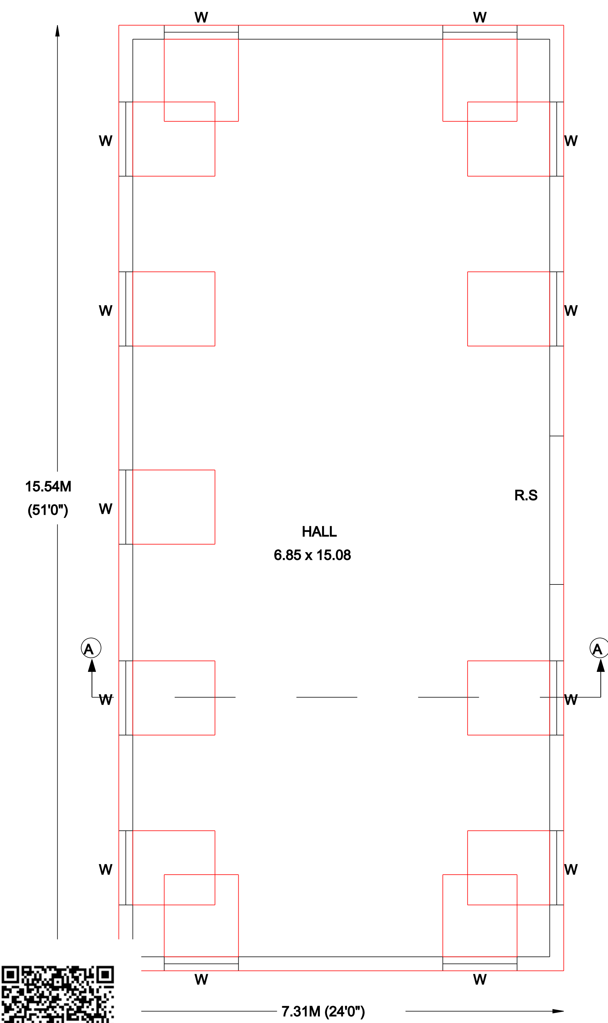
PROPOSED ADDITIONAL GROUND FLOOR PLAN
