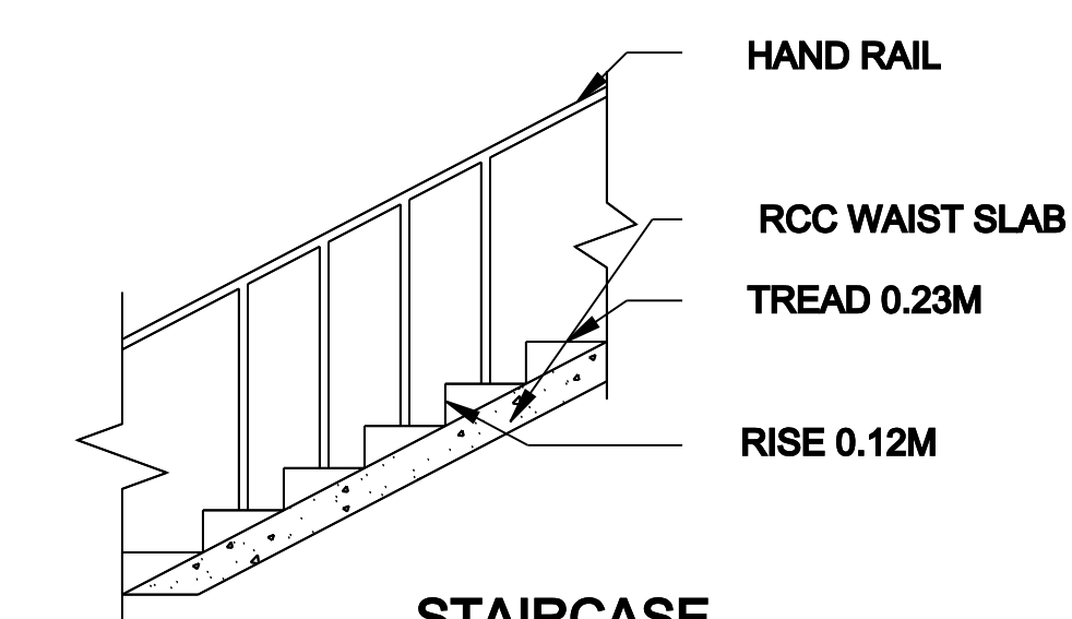
STAIRCASE
