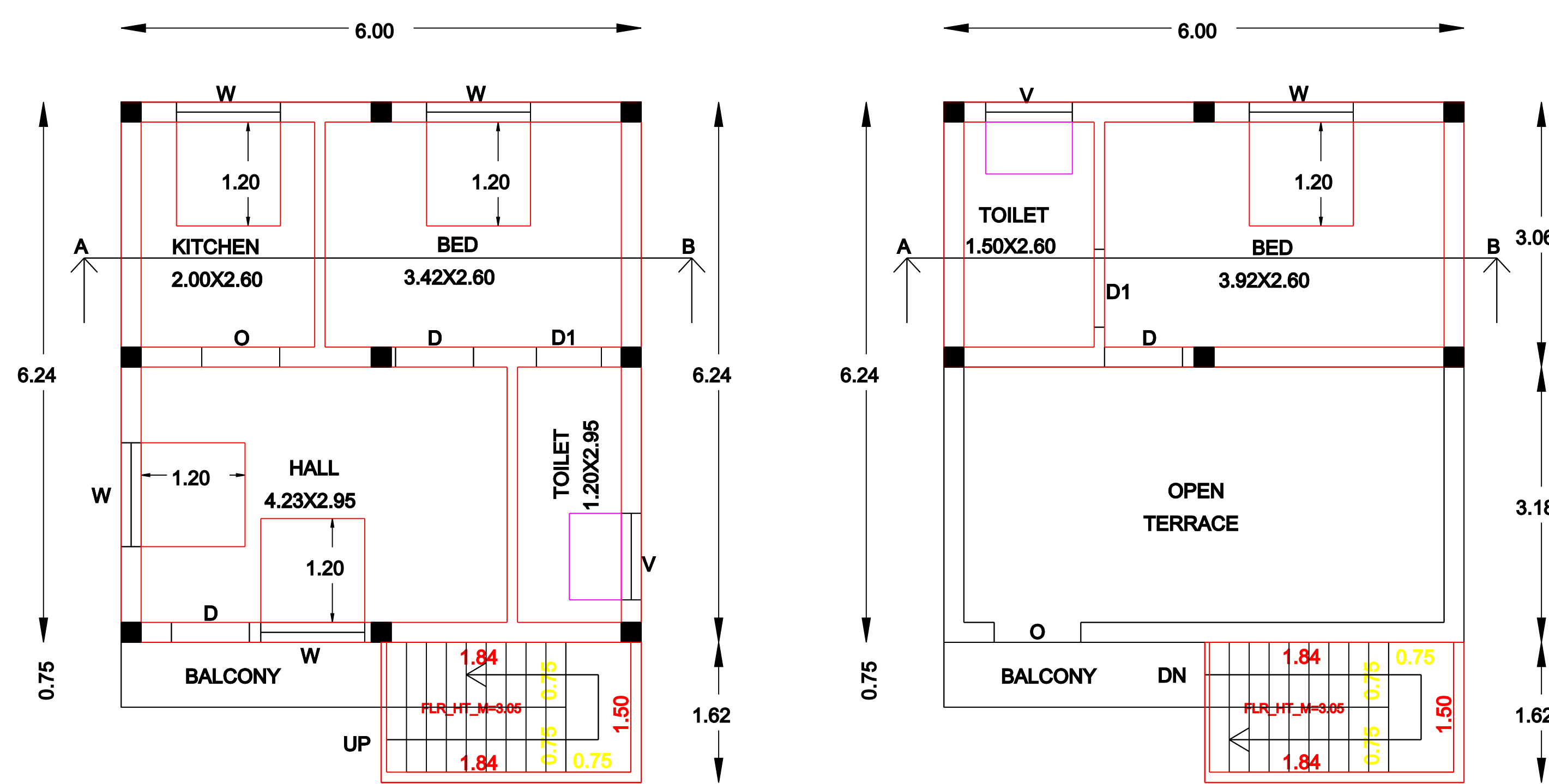
GF PLAN
