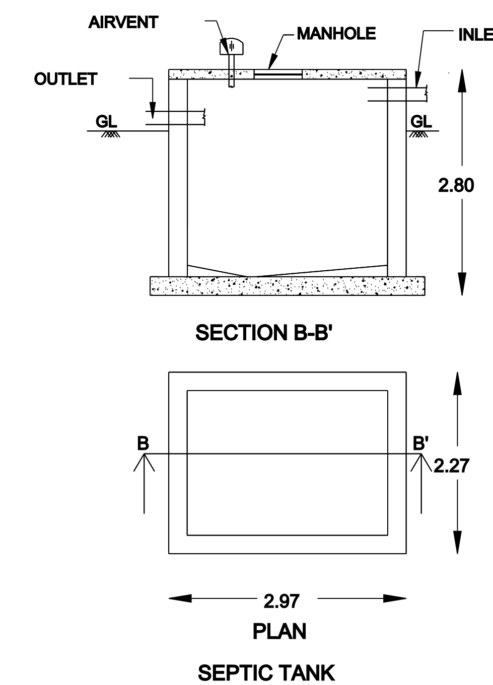
SEPTIC TANK
