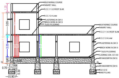
SECTION ON 'X-Y'
