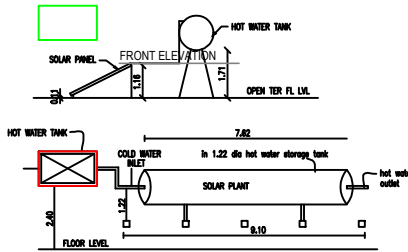
SOLAR WATER HEATER PLANT DETAILS
