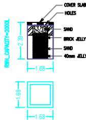
RAIN WATER COLLECTION TANK
