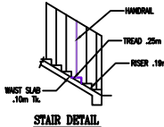
STAIR DETAIL
