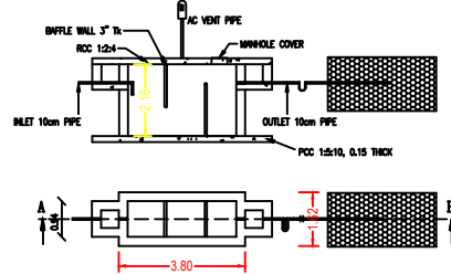
SEPTIC TANK AND TRENCH & U TRAP
