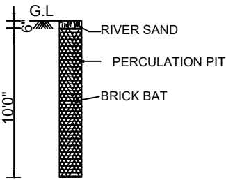
PERCULATION PIT
