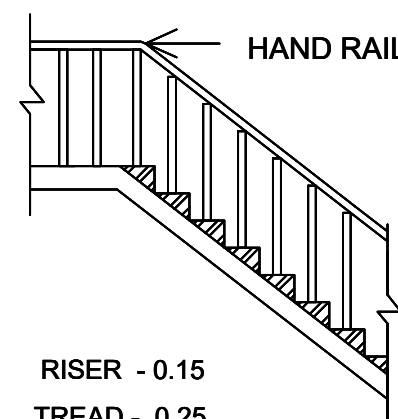
WIDTH - 0.76 STAIRCASE DETAILS:-
