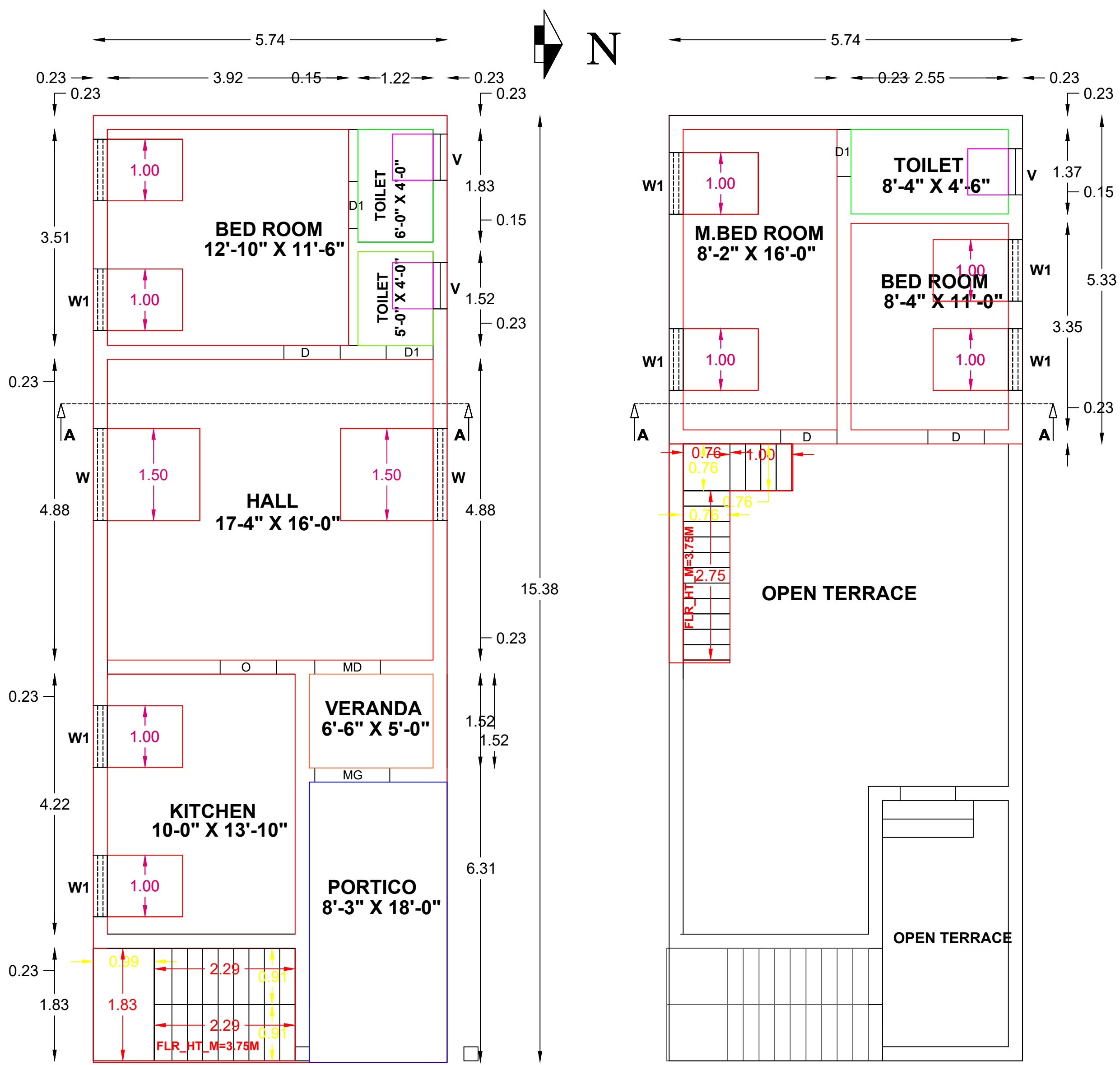
FLOOR PLAN
