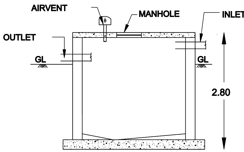
SECTION B-B'
