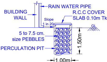
RAIN WATER HARVESTING TRENCH PIT DETAILS
