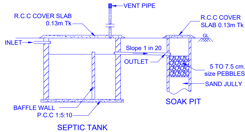
SEPTIC TANK DETAILS
