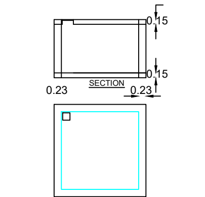
PLAN DETAILS OF COLLECTION SUMP FOR RAIN WATER HARVESTING OF ROOF TOP RAIN WATER
