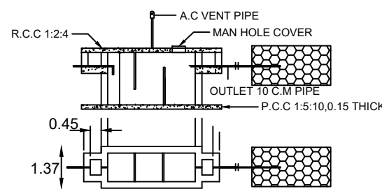
SEPTIC TANK DETAILS
