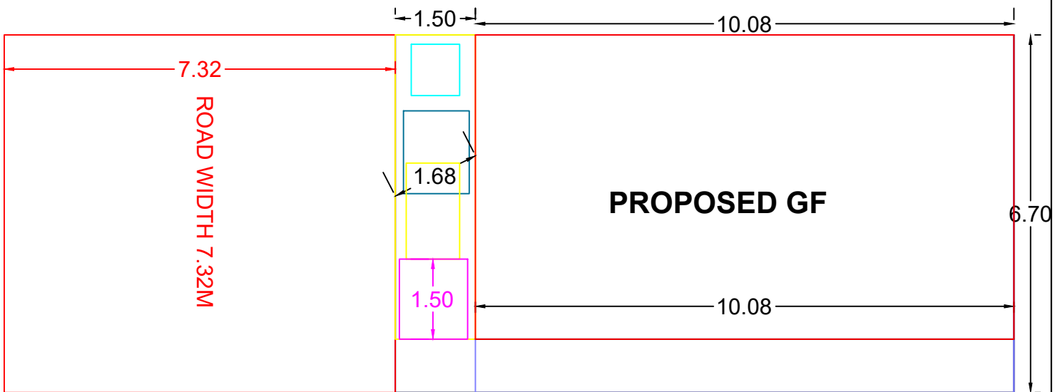
SITE PLAN
