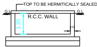
RWH SECTION (SAMPLE)
