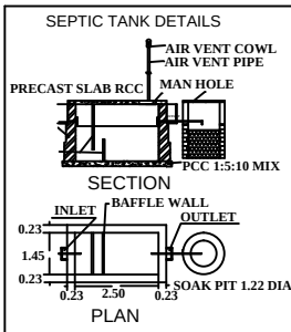
SEPTIC TANK DETAILS
