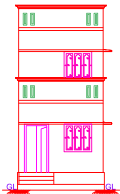
FRONT ELEVATION
