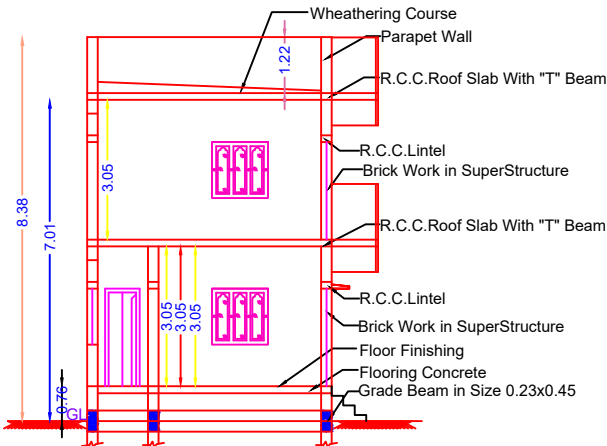
SECTION ON "PQ"
