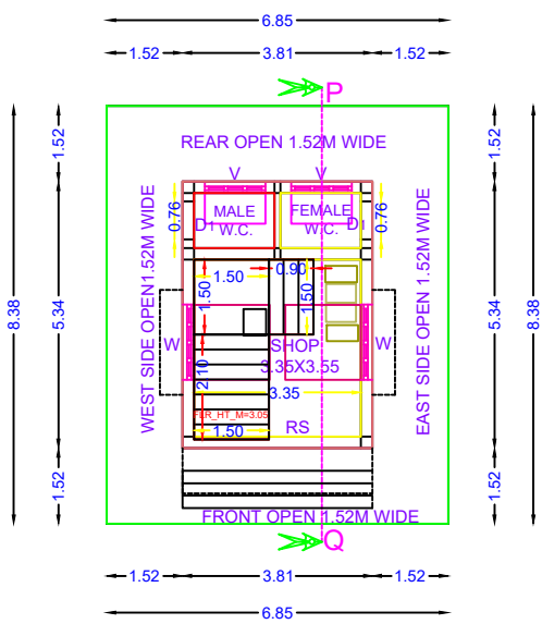
GROUND FLOORPLAN
