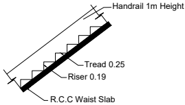
STAIR DETAILS
