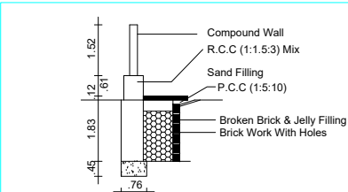
RAIN WATER HARVEST DETAILS
