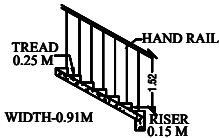
STAIRCASE DETAILS
