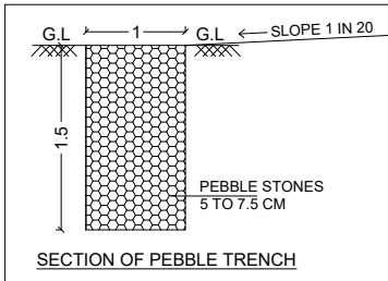
SECTION OF PEBBLE TRENCH
