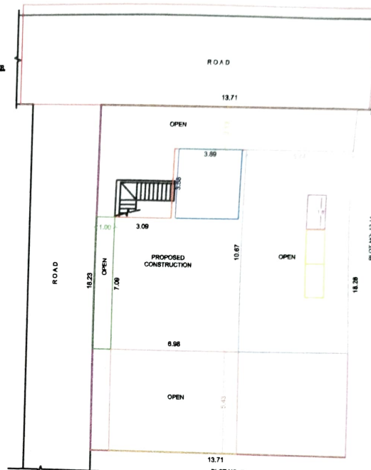
SITE PLAN
