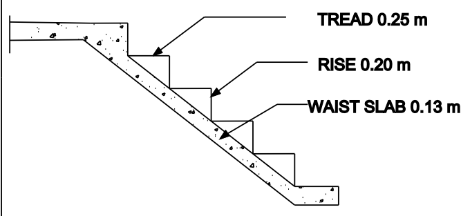
STAIR DETAILS
