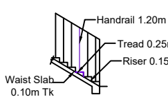
DETAILS OF STAIR CASE (SCALE 1:100)
