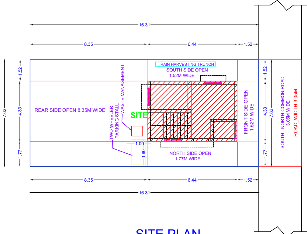
SITE PLAN
