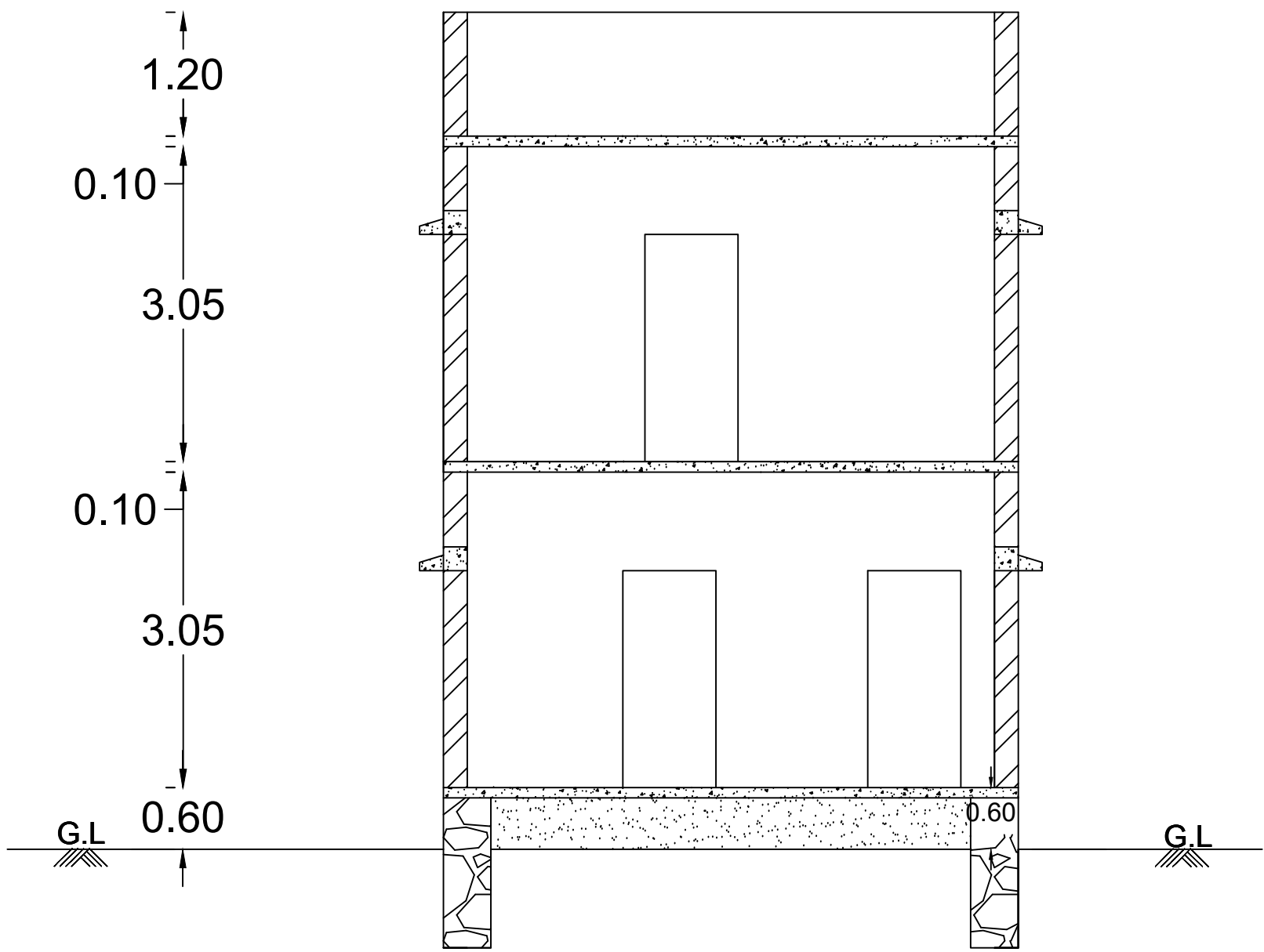
SECTION - AA
