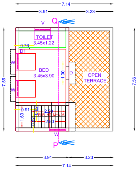
FRIST FLOOR PLAN
