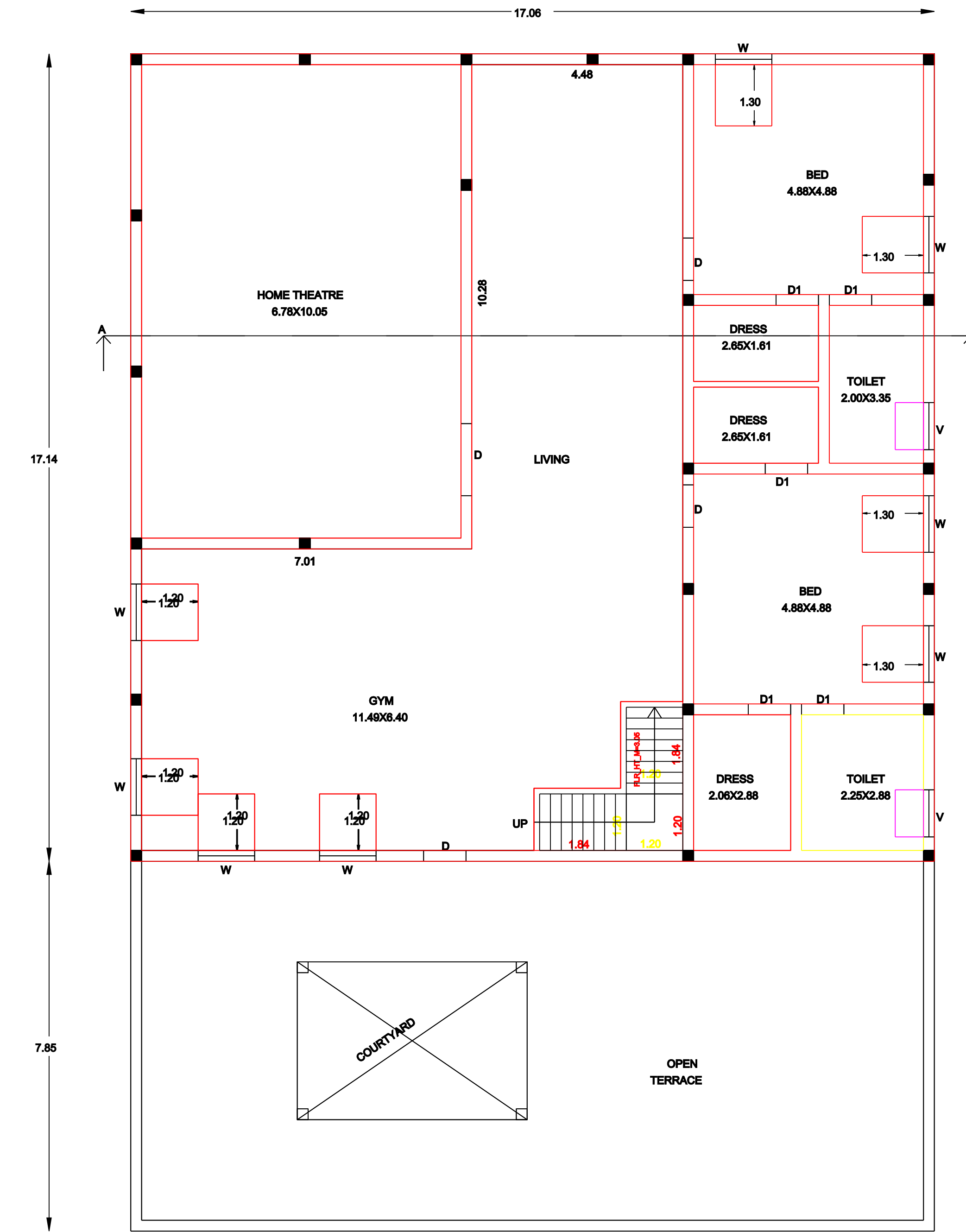
FF PLAN
