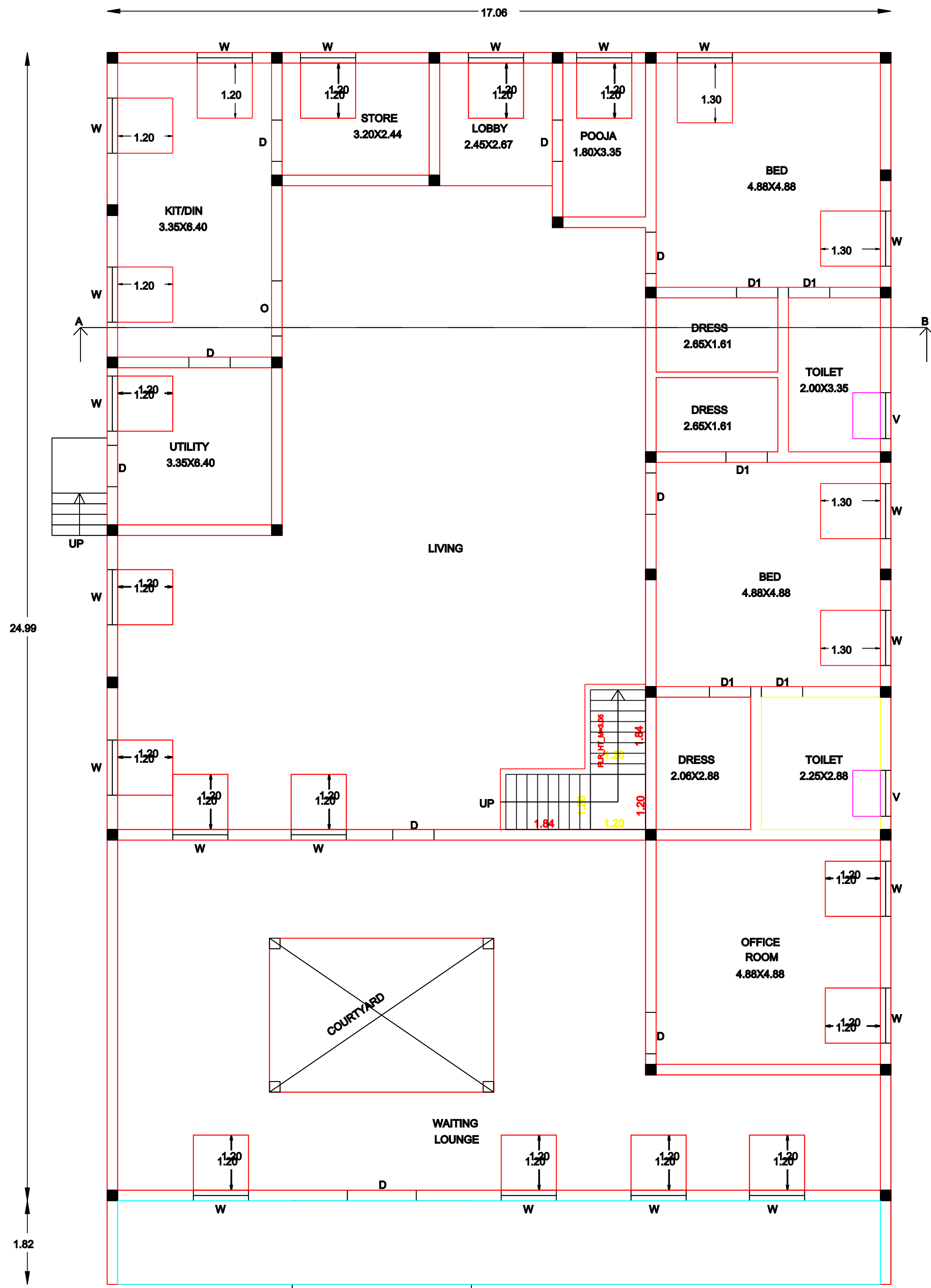
GF PLAN
