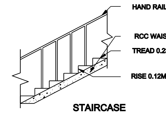
STAIRCASE
