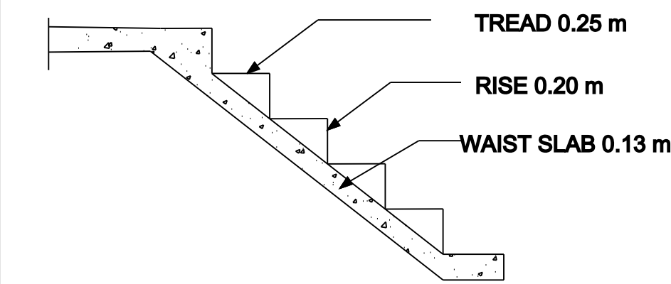
STAIR DETAILS
