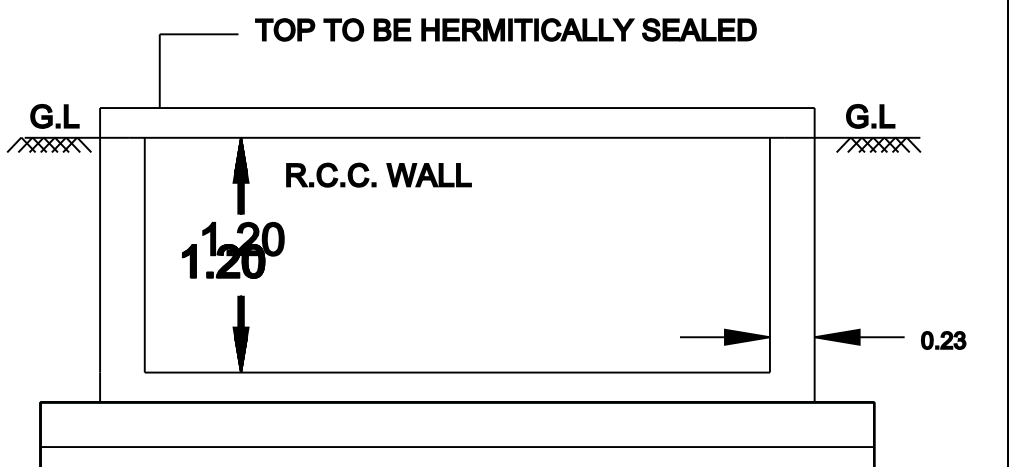
RWH_CAPACITY_L = 2000 RW SECTION
