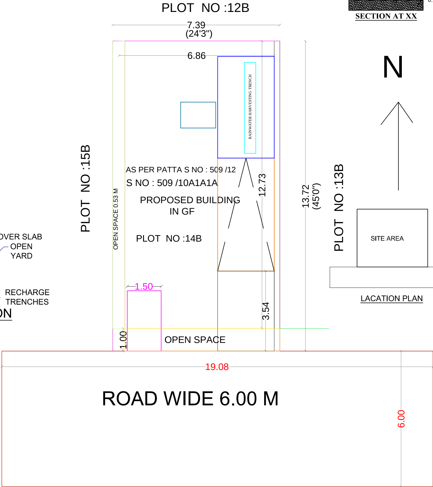
SITE PLAN
