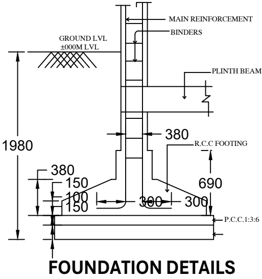
FOUNDATION DETAILS
