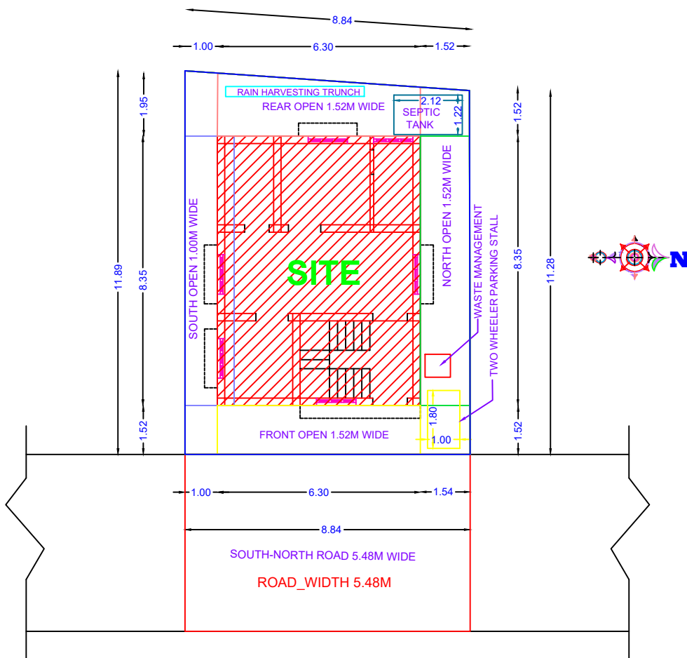
SITE PLAN
