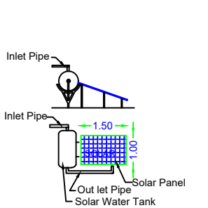
DETAILS OF SOLAR WATER HEATER
