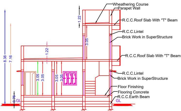
SECTION ON "PQ"
