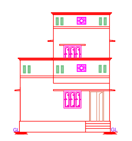
FRONT ELEVATION
