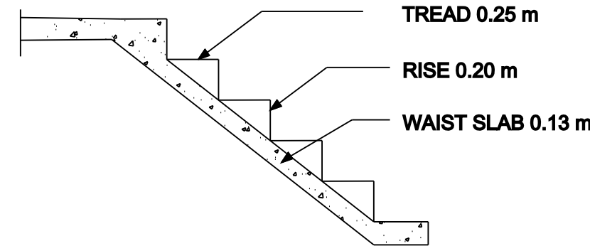
STAIR DETAILS
