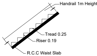
STAIR DETAILS
