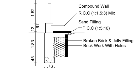
RAIN WATER HARVEST DETAILS
