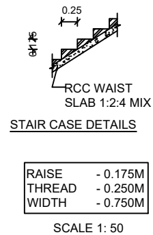
SCALE 1: 50
