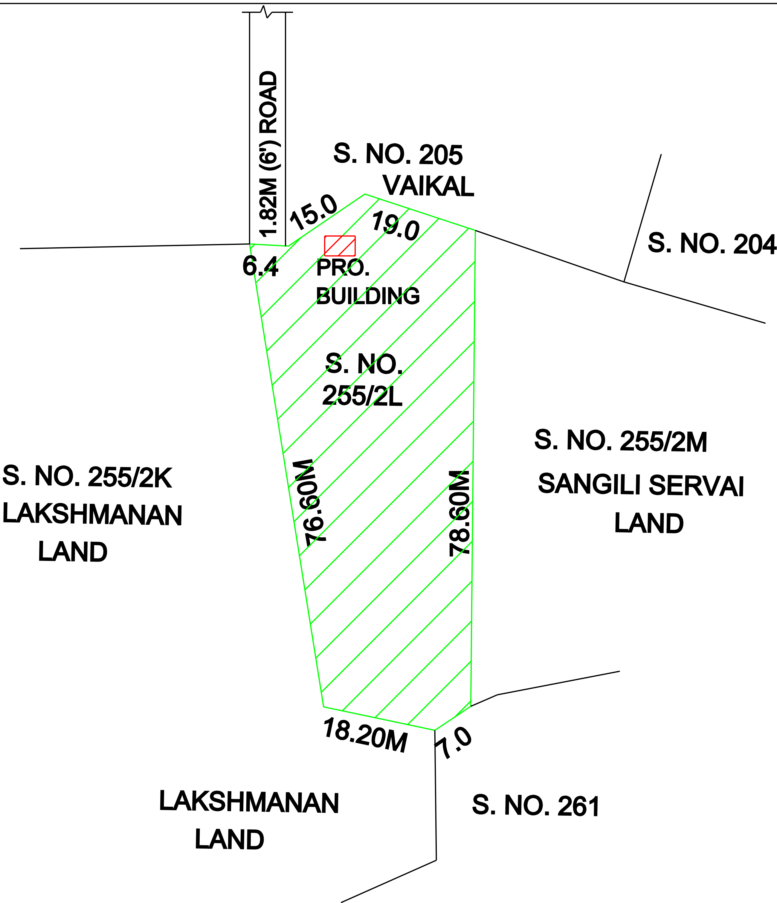
LOCATION PLAN
