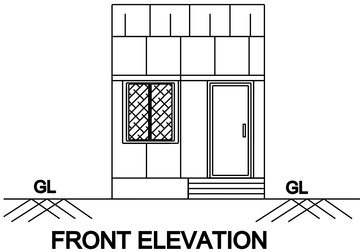
FRONT ELEVATION
