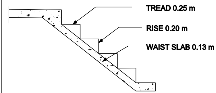
STAIR DETAILS
