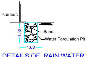
DETAILS OF RAIN WATER PERCOLATION PIT
