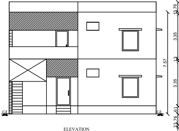
ELEVATION 10.88
