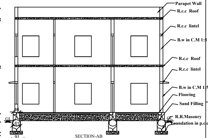
SECTION-AB 10.88
