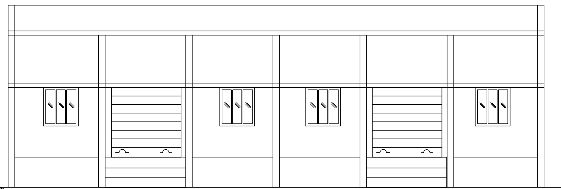
EASTERN SIDE ELEVATION
