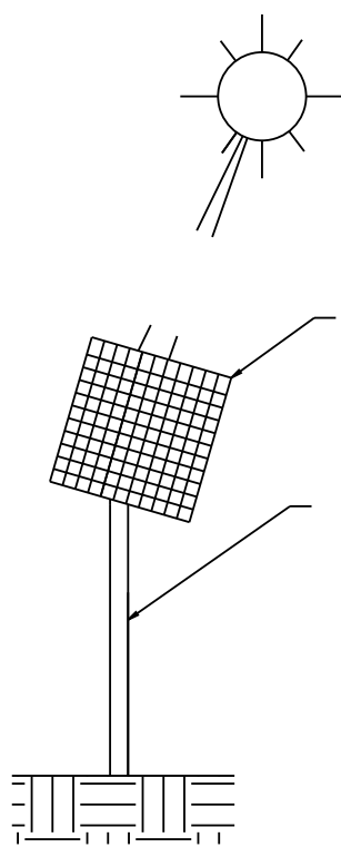
SOLAR SYSTEM
