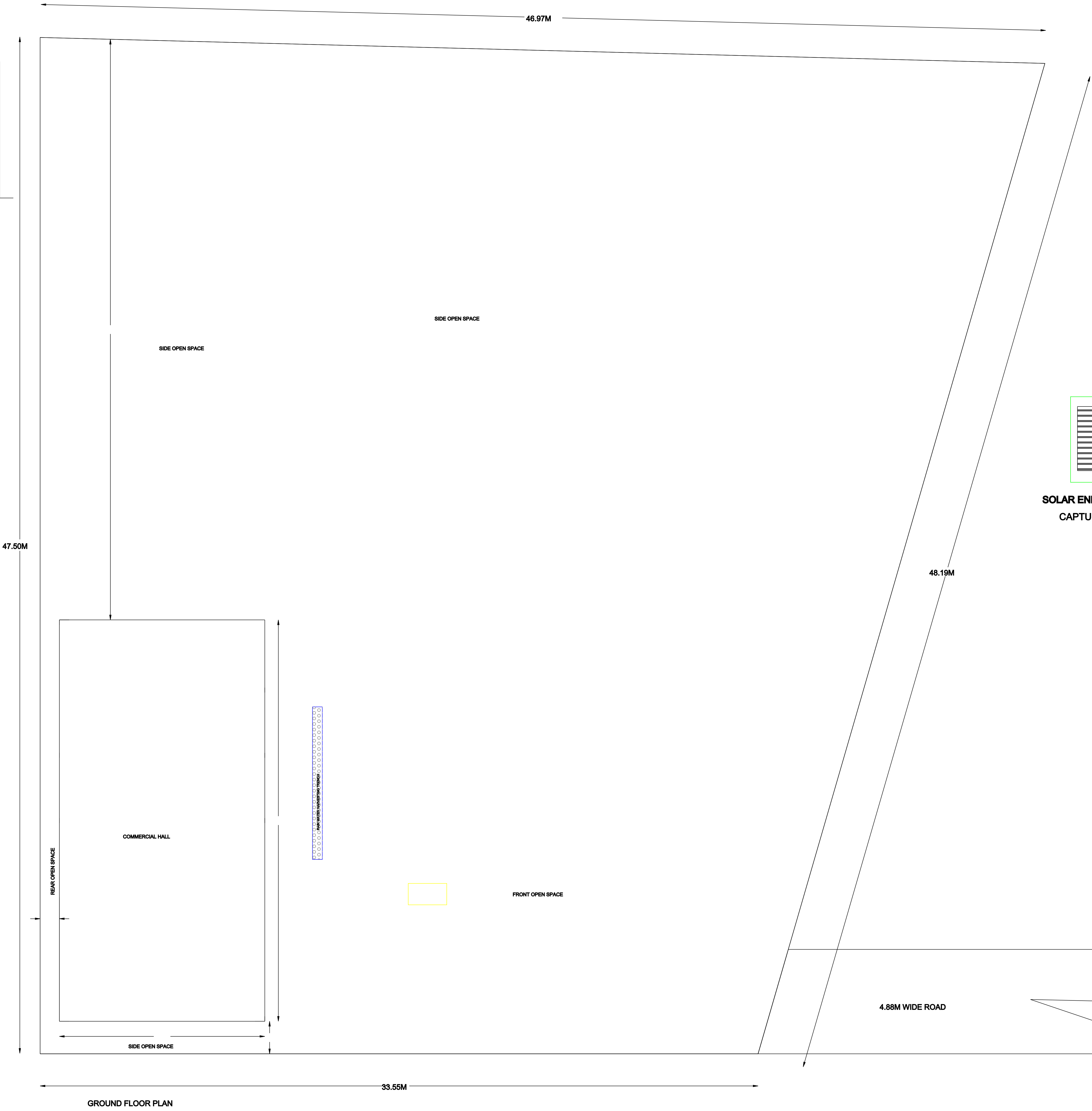
SOLAR SYSTEM
