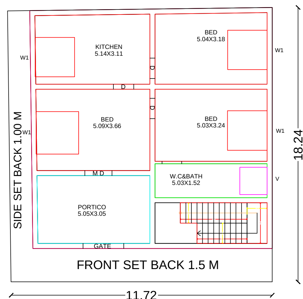
FLOOR PLAN
