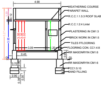
SECTION ON 'XY'
