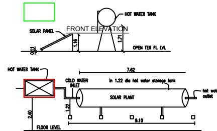
SOLAR WATER HEATER PLANT DETAILS
