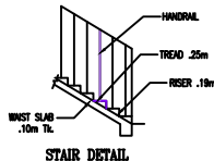
STAIR DETAIL
