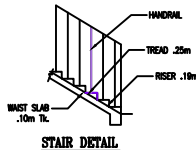
STAIR DETAIL
