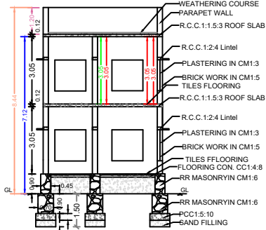
SECTION ON 'XY'
