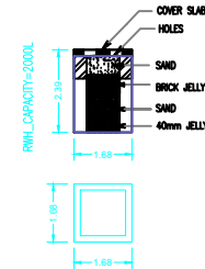
RAIN WATER COLLECTION TANK
