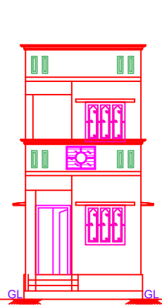
FRONT ELEVATION
