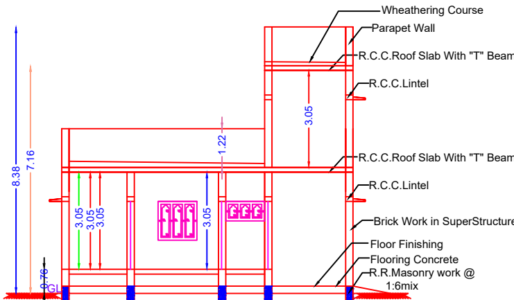
SECTION ON "PQ" SCALE 1:100
