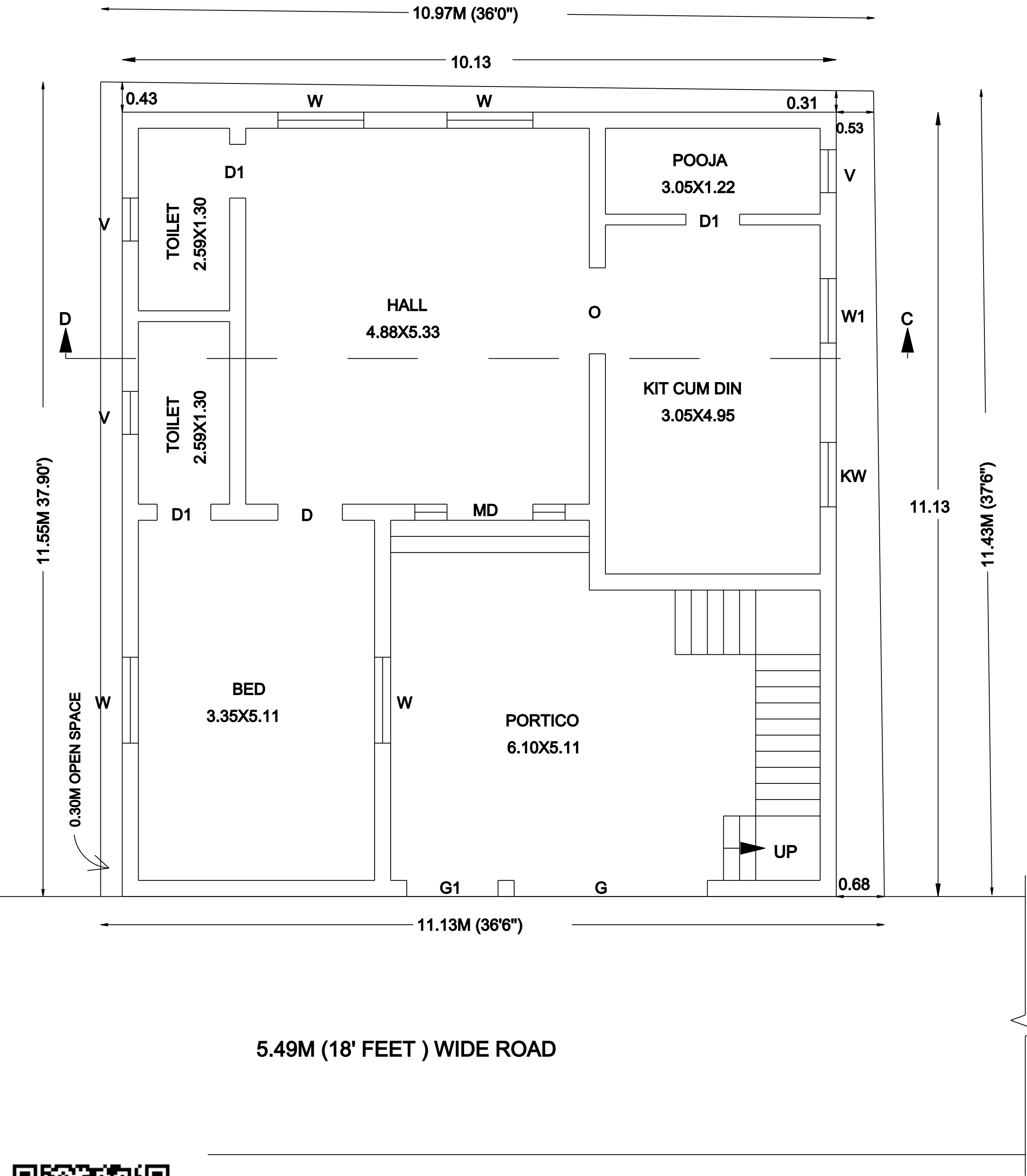
GROUND FLOOR PLAN (EXISTING)
