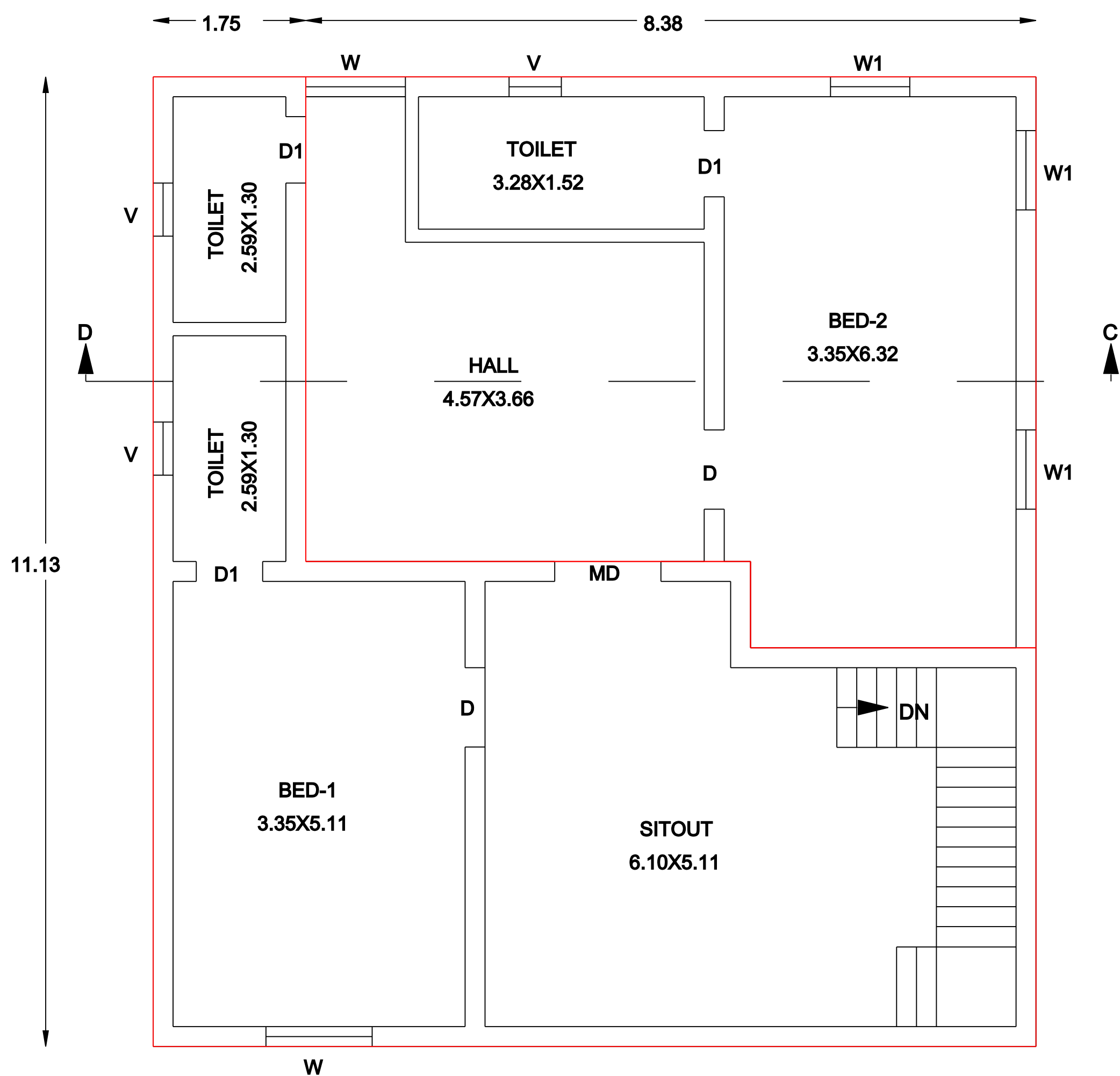
FIRST FLOOR PLAN (EXISTING & PROPOSED)
